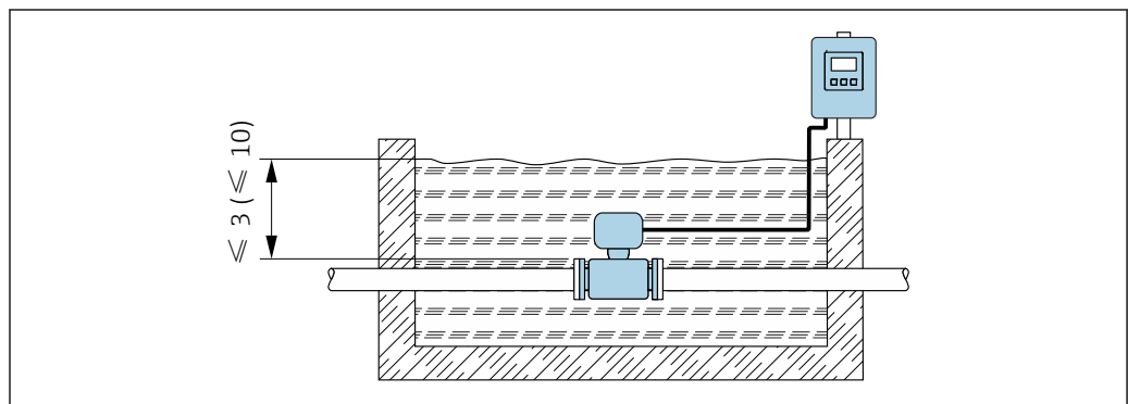
36 Engineering unit in m(ft)
