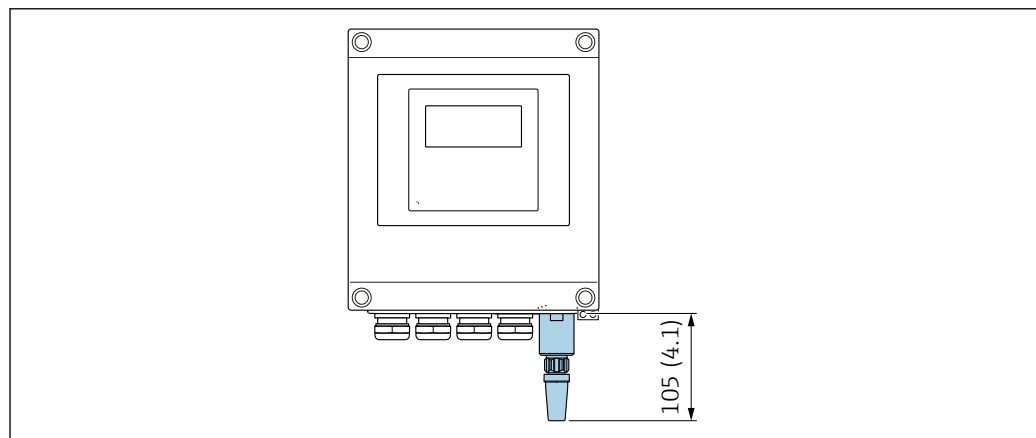
56 Engineering unit mm (in)
