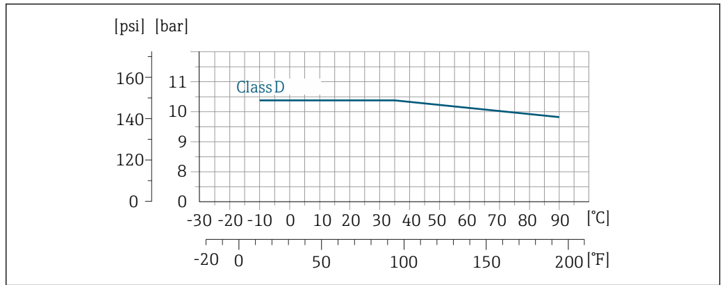
41 Process connection material: carbon steel
