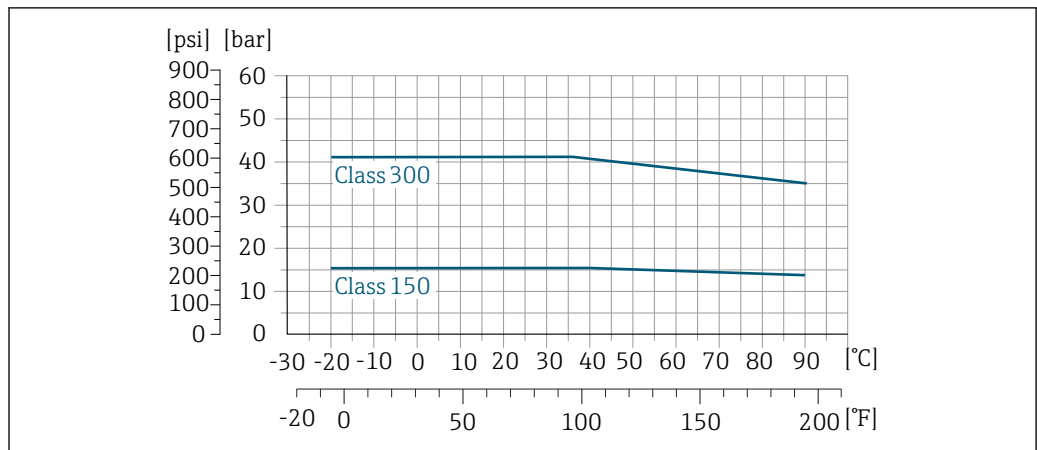
38 Process connection material: stainless steel
