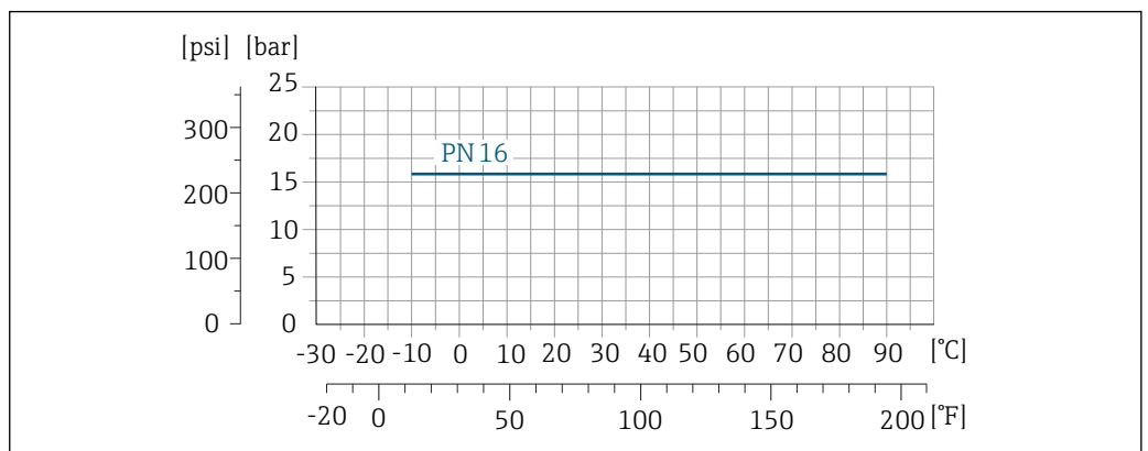
43 Process connection material: carbon steel
