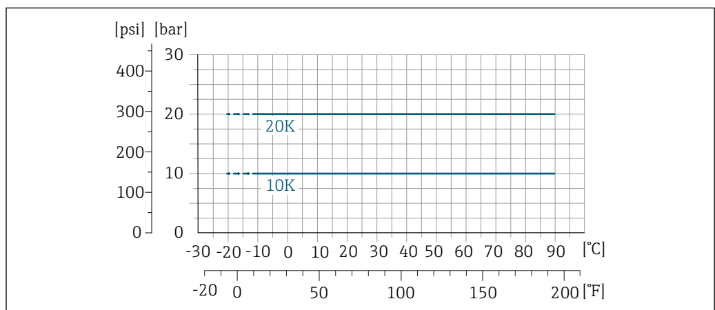
40 Process connection material: stainless steel (-20 °C (-4 °F)); carbon steel (-10 °C (14 °F))
