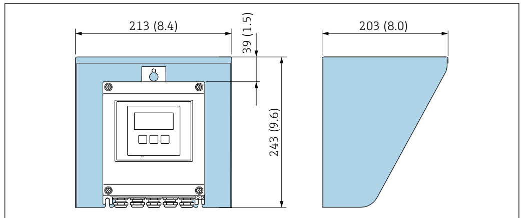
54 Weather protection cover for Proline 500 – digital
