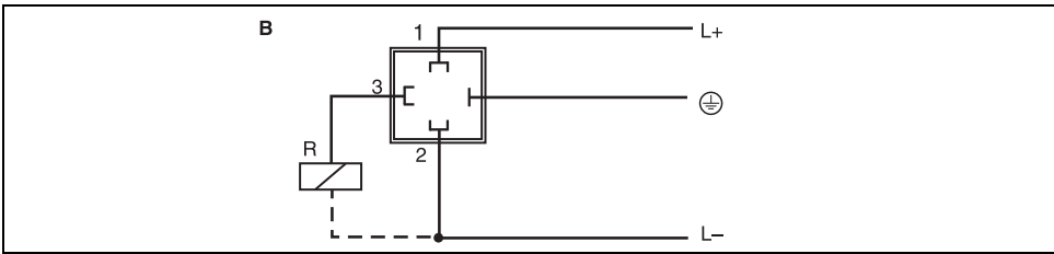
Fig. 9: Flowphant® T with M16x1.5 valve connector or NPT ½"
