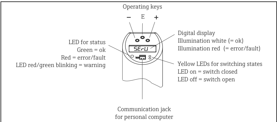
Fig. 10: Position of operating elements and possibilities for display
