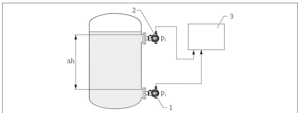
Level measurement in a closed tank with pressure overlay
