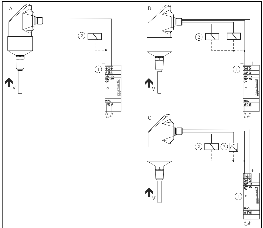
A: 1x PNP switch output B: 2x PNP switch output C: PNP switch output with additional analog output 4 to 20 mA
