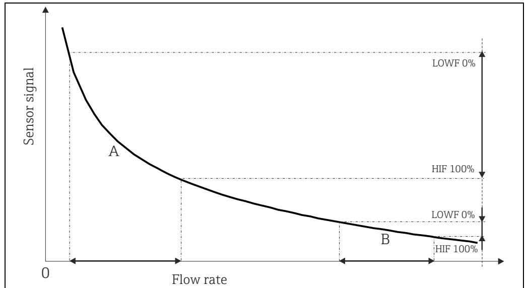
Standard characteristic
