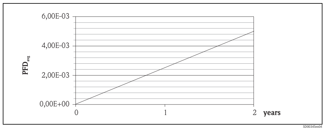
Proof-test interval
