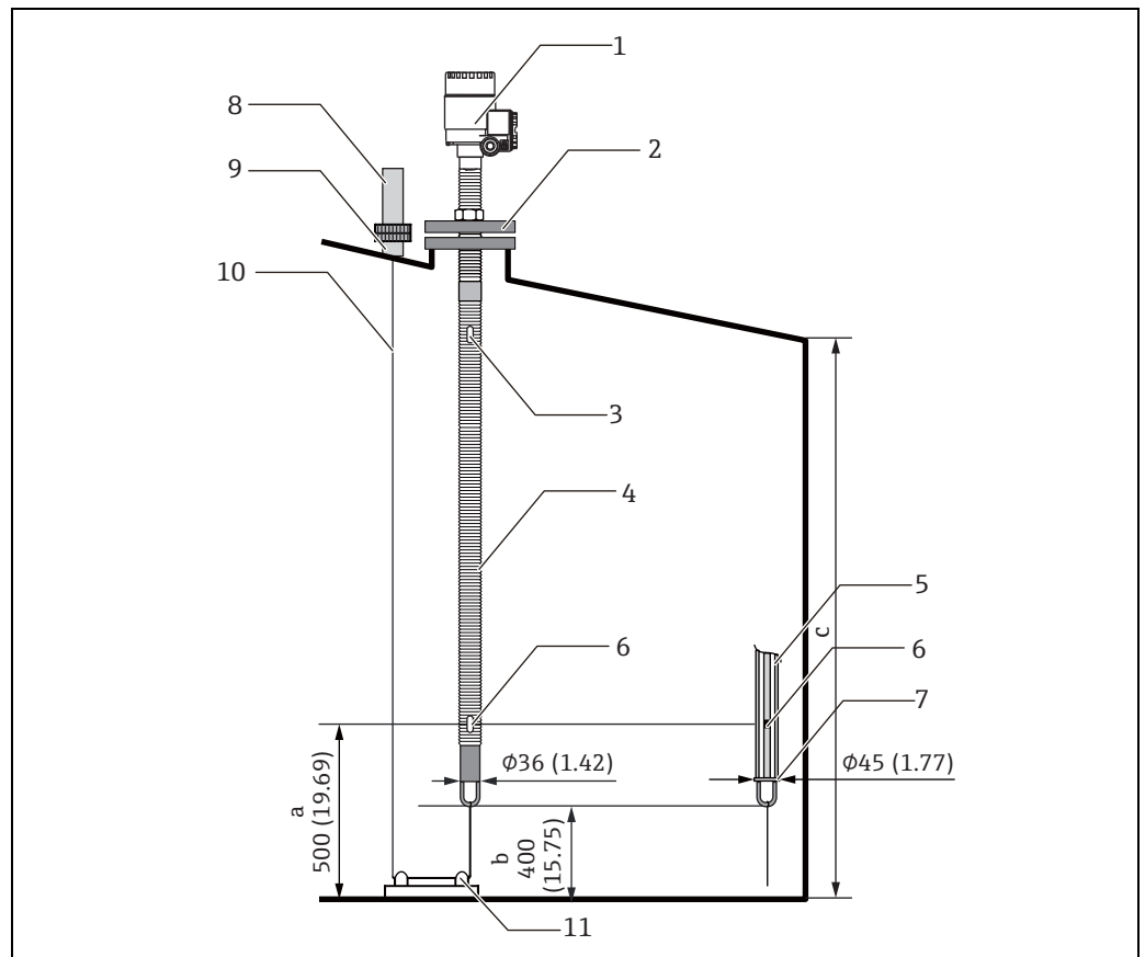
Figure 23: Top anchor method, Unit of measurement: mm (in)
