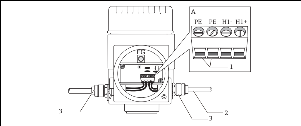
Figure 43: NMT539 terminal (TIIS Ex d [ia]) A Temperature (water bottom sensor) data/Intrinsically safe HART on NMT539 (See Tips). 1 Non-hazardous area, Class A grounding (1 to 1.5 mm 2 , 2pcs.) 2 Screened twisted pair or steel armored wire 3 Cable gland (SXC-16B)
