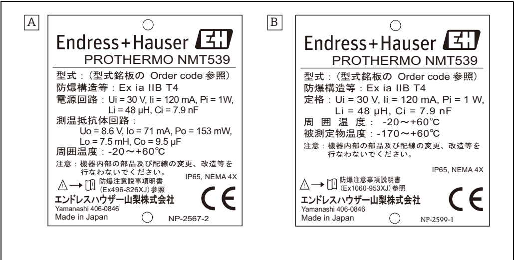
Figure 3: TIIS Ex ia approval nameplate 2 A Only for transmitter (TIIS number: TC18321) B NMT539 for low temperature (TIIS number: TC18604)1
