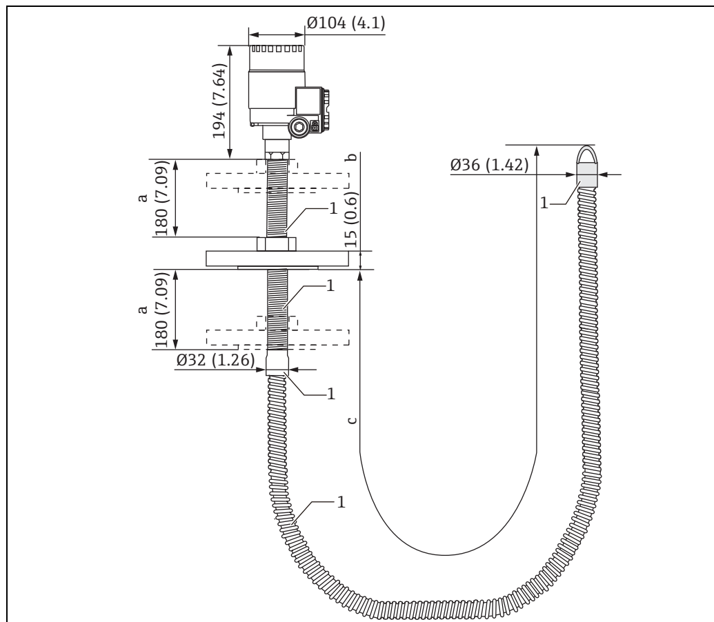
Figure 13: Dimensions for converter + average + temperature prob, Unit of measurement: mm (in)
