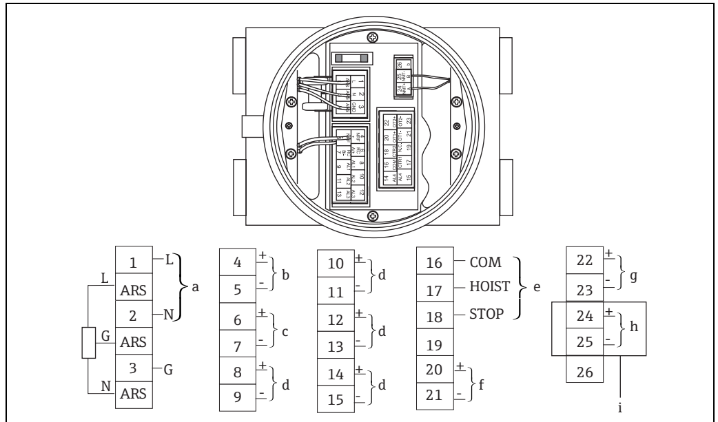
Figure 44: NMS Ex d connection
