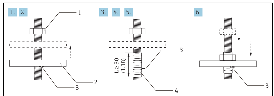
Figure 20: Wrapping Sealing Tape, Unit of measurement: mm (in)
