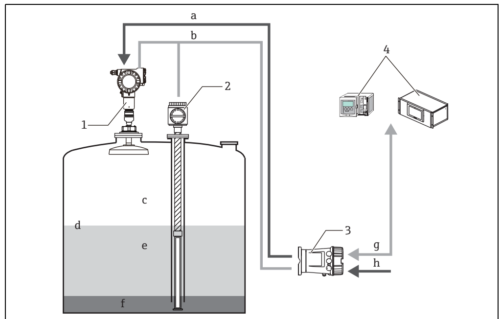
Figure 53: System layout NMT539 Ex ia + NRF81 Ex d [ia]
