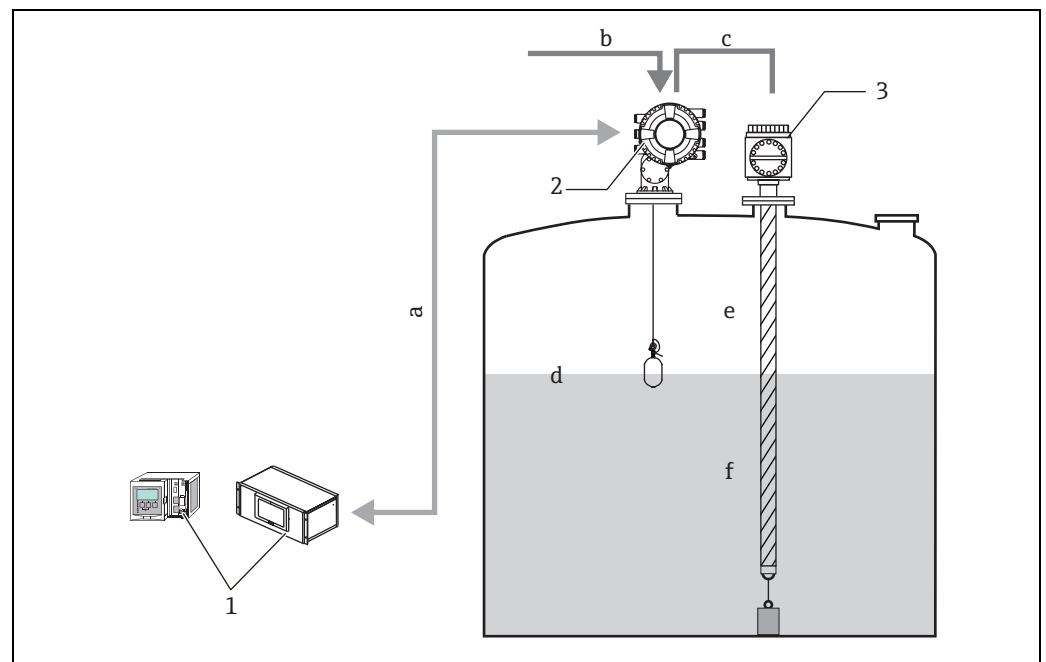
Figure 51: System layout (ATEX, FM, CSA, Ex i) with NMS5 and NMS8x
