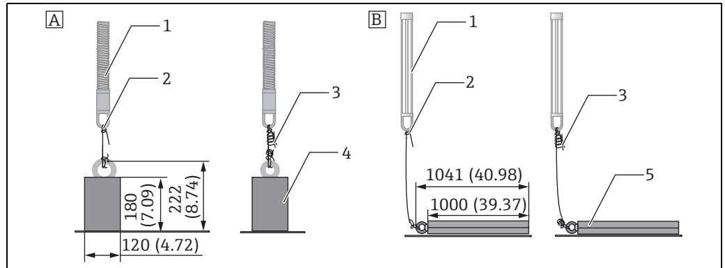
Figure 28: Anchor weight attachment, Unit of measurement: mm (in)
