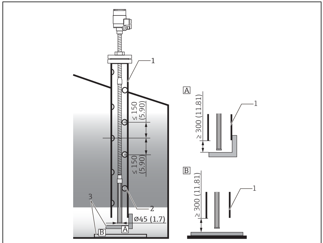
Figure 26: Stilling well method, Unit of measurement: mm (in)
