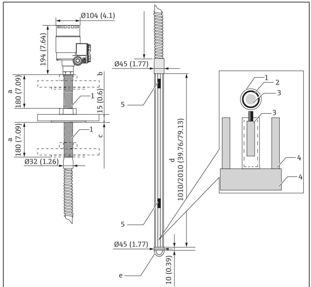
Figure 14: Dimension of Converter + average temperature probe + WB probe, Unit of measurement: mm (in)
