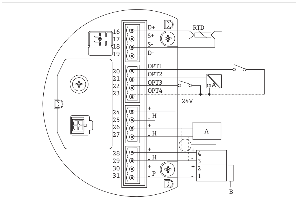
Figure 45: NRF590 terminals (Ex ia)
