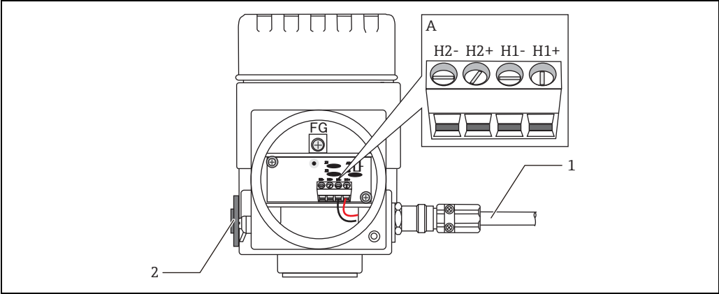
Figure 40: NMT539 Terminals (ATEX, Ex ia) A Temperature (water bottom sensor) data/Intrinsically safe HART on NMT539 (See Tips). 1 Screened twisted pair or steel armored wire 2 Blind plug (standard aluminum)
