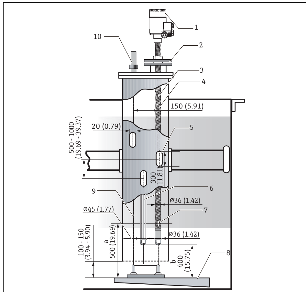
Figure 29: Top anchor method, Unit of measurement: mm (in)
