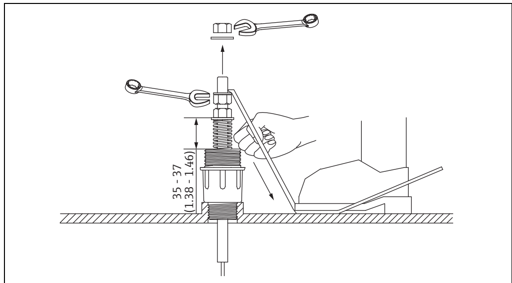
Figure 25: Top anchor attachment-2, Unit of measurement: mm (in)
