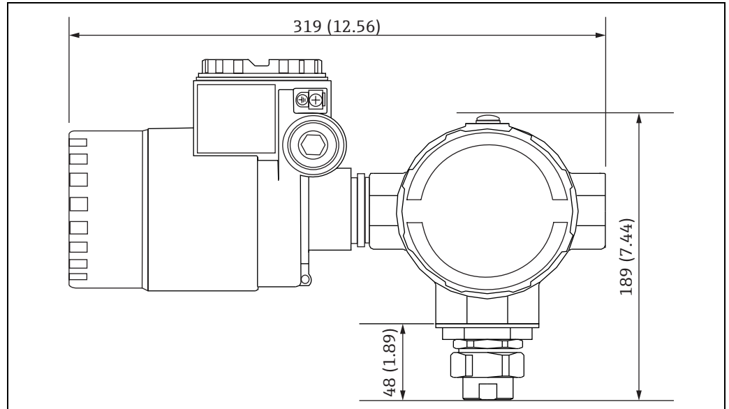
Figure 11: Converter only (standard PF (NPS) 3/4 universal coupling connection), Unit of measurement: mm (in)
