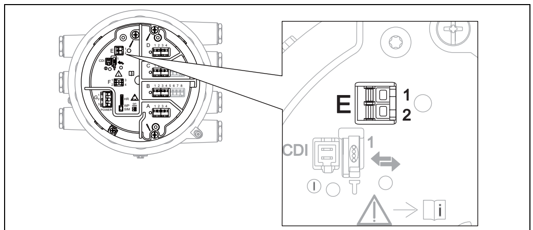
Figure 42: NMS8x terminal for NMT539
