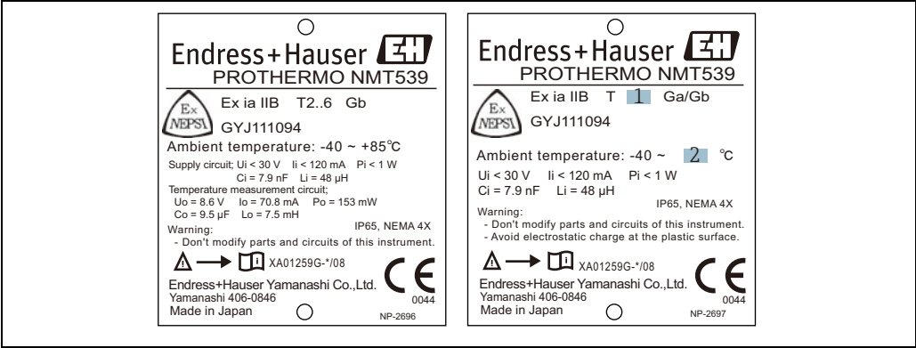
Figure 10: NEPSI approval nameplate
