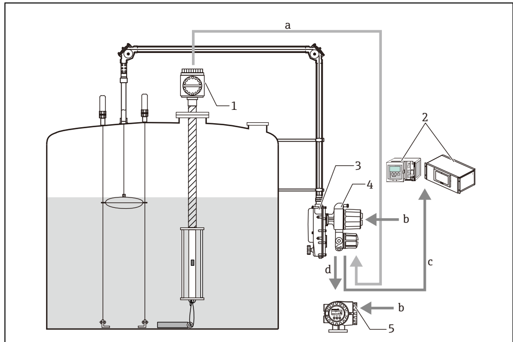
Figure 54: System layout NMT539 Ex d [ia] + TMD1 Ex d
