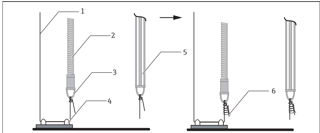
Figure 24: Top anchor attachment-1
