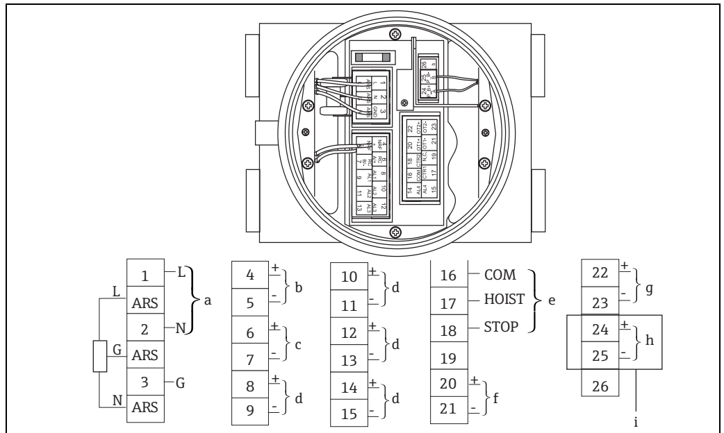
Figure 41: NMS5 terminal
