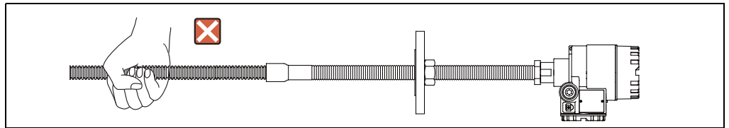
Figure 17: Handling of flexible tube
