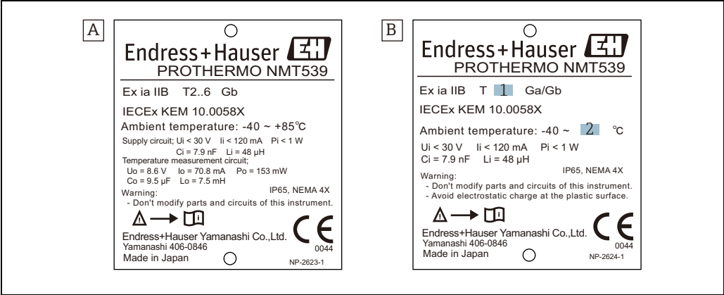
Figure 9: IEC approval nameplate
