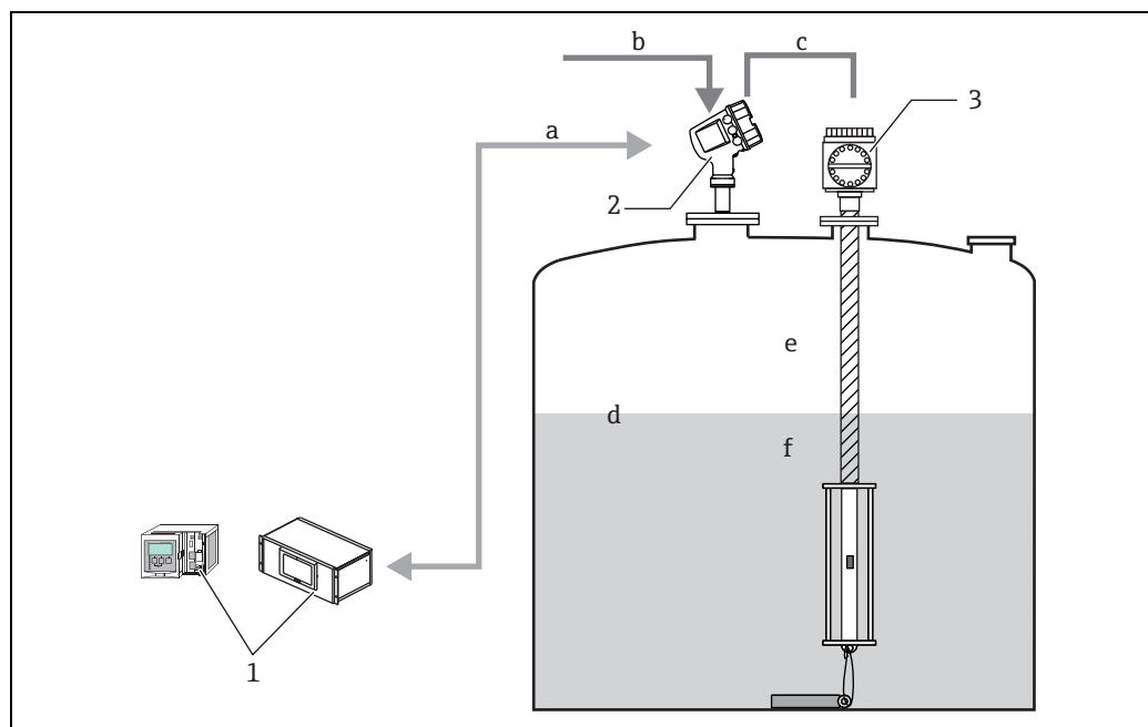
Figure 52: System layout NMT539 Ex ia + NMRx Ex d [ia]
