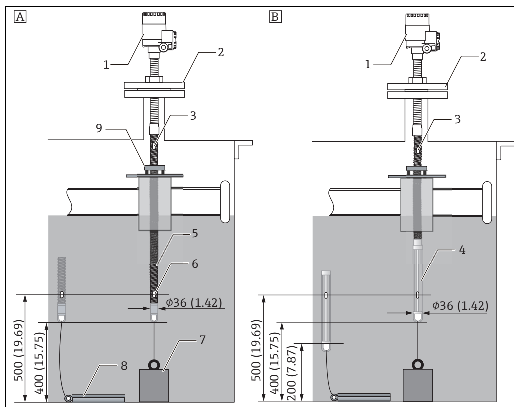
Figure 31: Guide ring and anchor weight, Unit of measurement: mm (in)
