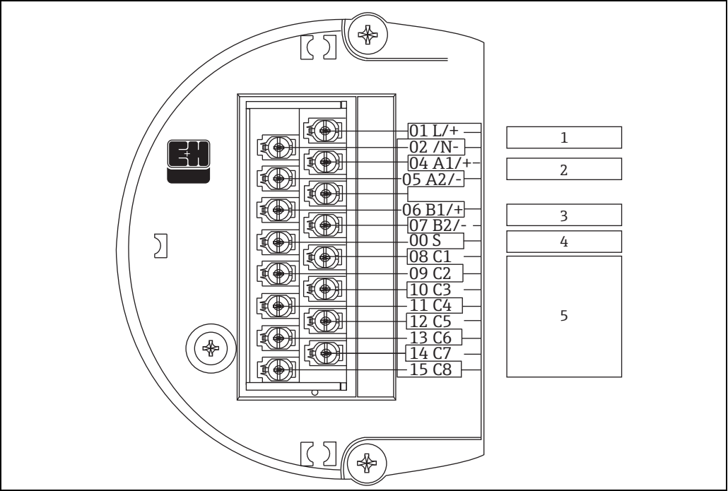
Figure 46: NRF590 terminals (TIIS Ex d)
