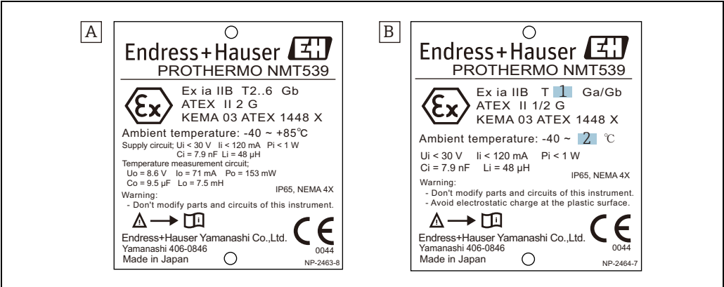
Figure 5: ATEX Ex ia approval A Converter B Average temperature and water bottom sensor 1. Temperature class 2. Maximum ambient temperature
