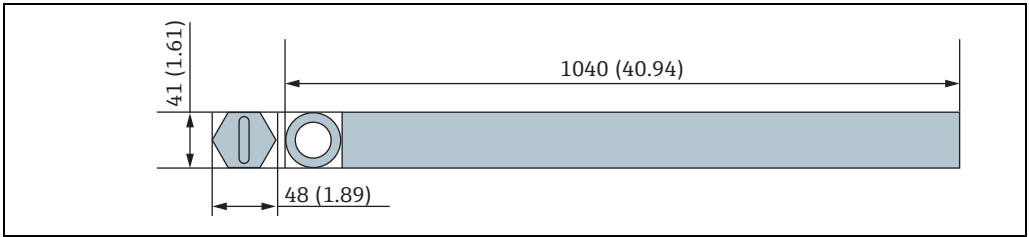
Figure 48: Anchor Weight for low profile, Option C and G, Unit of measurement: mm (in)
