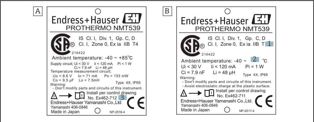
Figure 7: CSA approval nameplate
