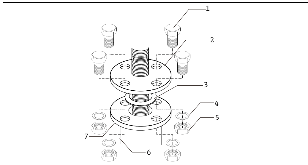
Figure 19: Mounting NMT539
