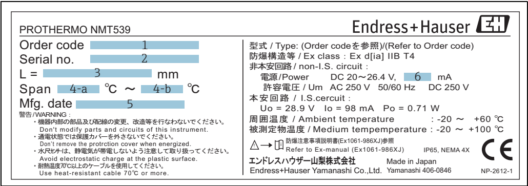
Figure 4: TIIS Ex d [ia] approval nameplate (TIIS number: TC18884) 1. Order code 2. Serial number 3. Flexible tube length 4. Measuring temperature range 5. Date of manufacture (MM/YY) 6. Consumption
