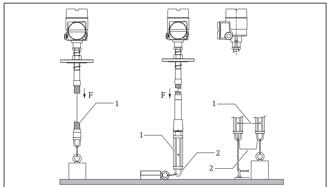
Figure 21: Mounting accessory
