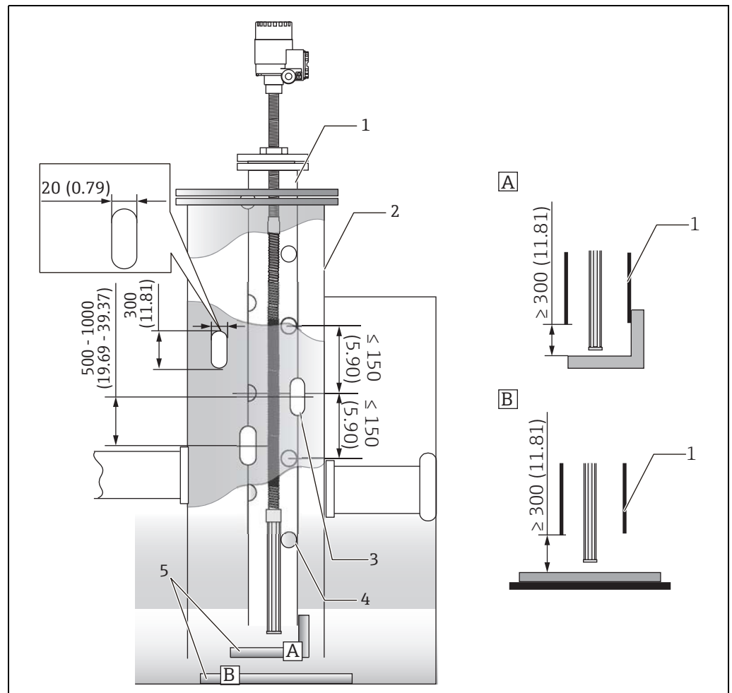
Figure 30: Stilling well method, Unit of measurement: mm (in)
