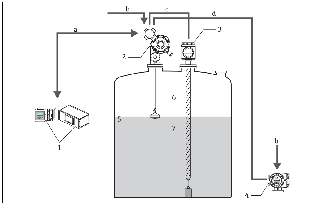
Figure 55: System layout NMT539 Ex d [ia] + TGM5 Ex d
