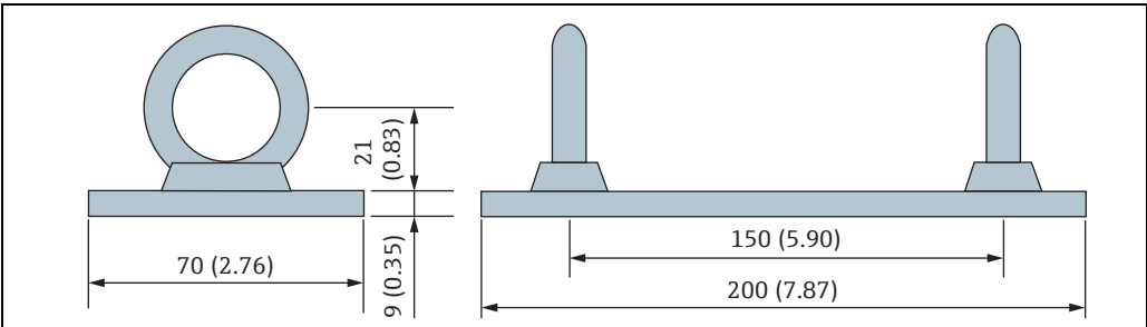
Figure 49: Wire hook, Option D and F, Unit of measurement: mm (in)
