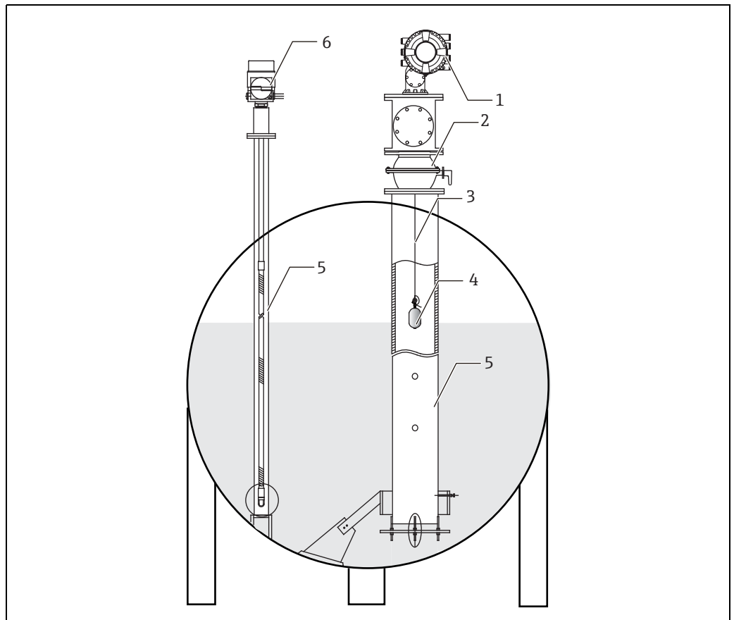
Figure 32: Stilling well for pressurized tank
