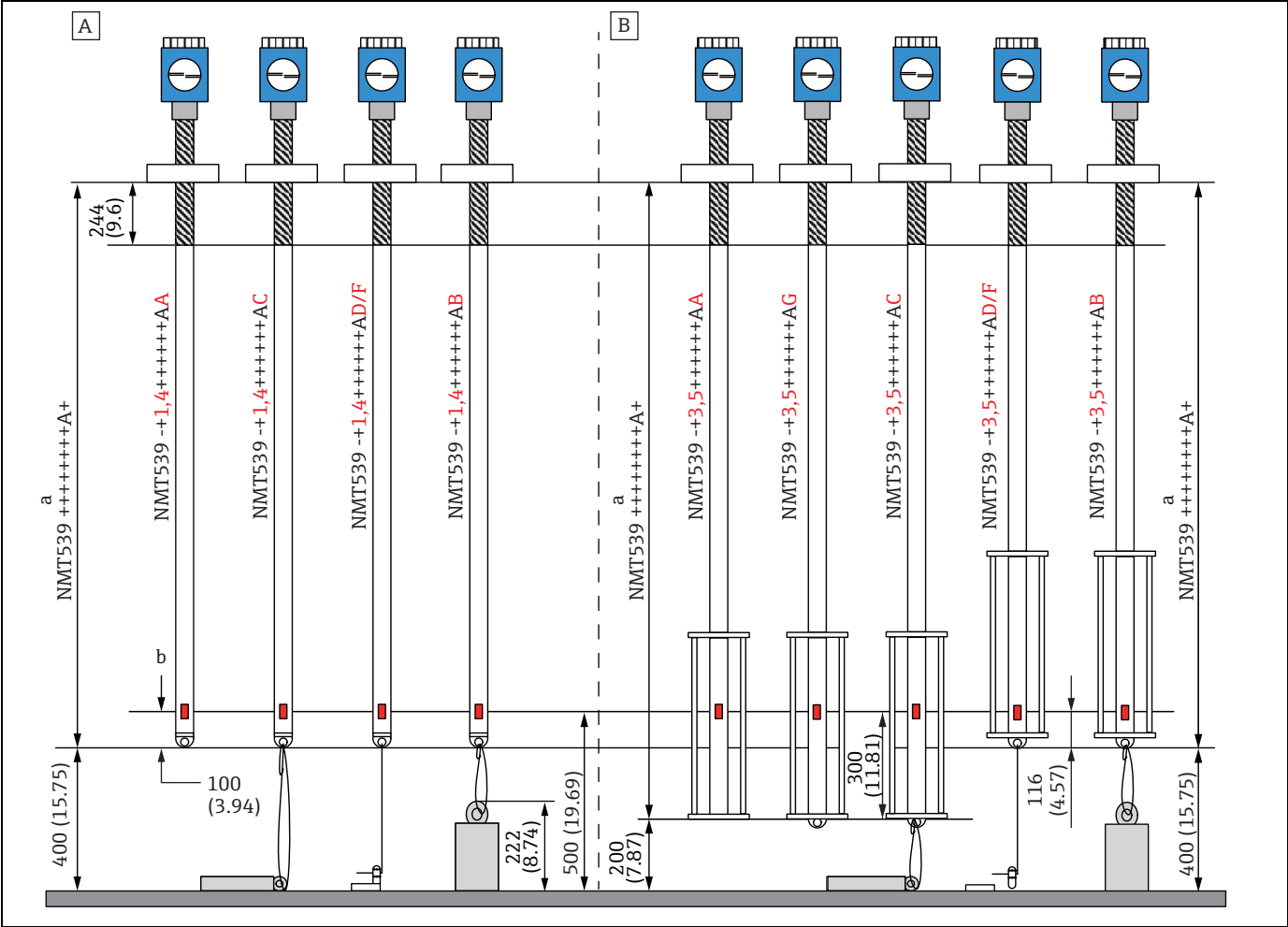
Figure 15:#1 Element Position, Unit of measurement: mm (in) A Transmitter + Temperature probe B Transmitter + Temperature probe + Water probe a Distance from the bottom of the flange b Position of No.1 element
