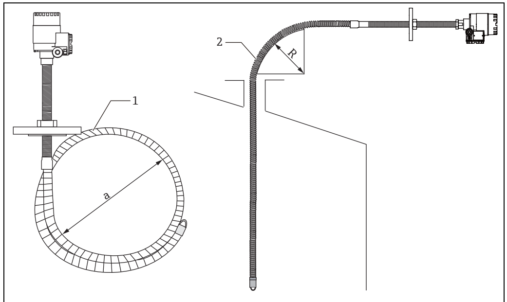
Figure 18: Handling of flexible tube 2, Unit of measurement: mm (in)
