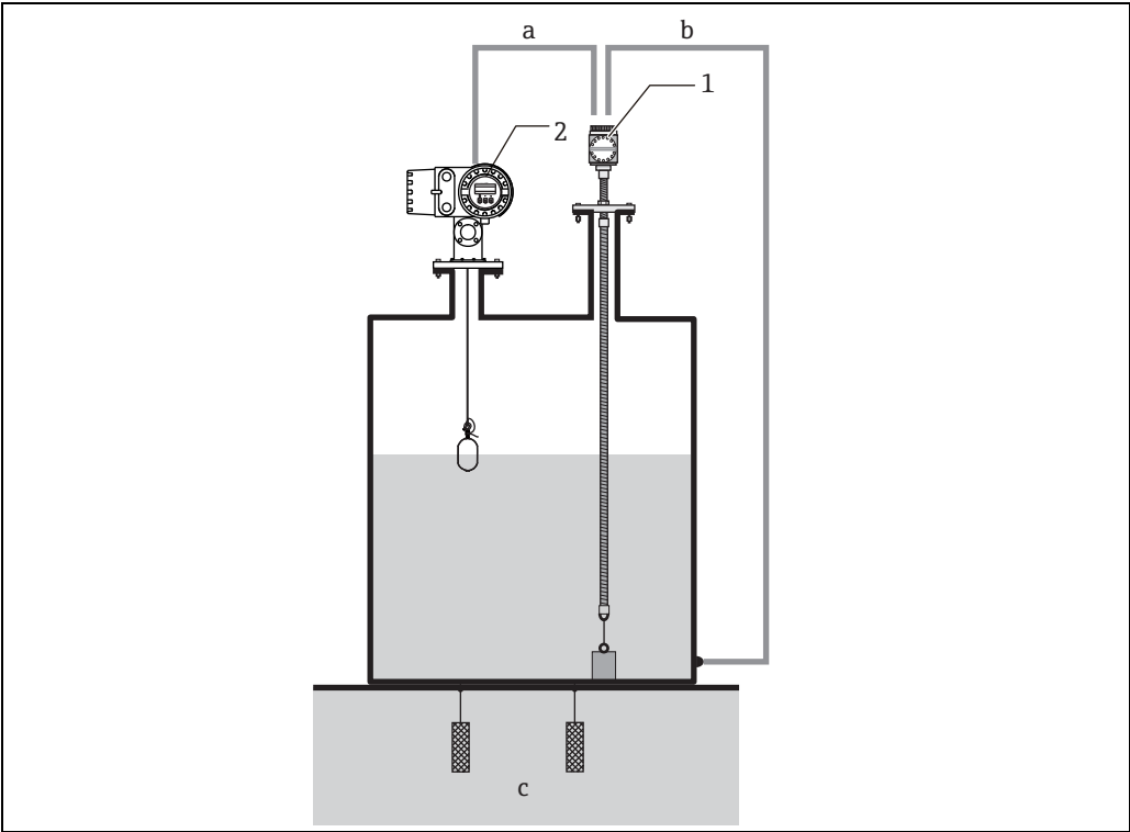
Figure 38: Grounding cable a Local HART (Ex d) communication b Grounding cable (see Tip.) c Non-hazardous area, Class A grounding, Under ground 1 NMT539 2 NMS5/NMS8x
