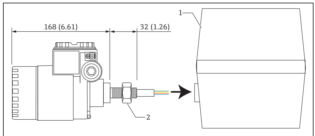
Figure 12: Converter only (for Varec 1700 with M20 threaded connection), Unit of measurement: mm (in)
