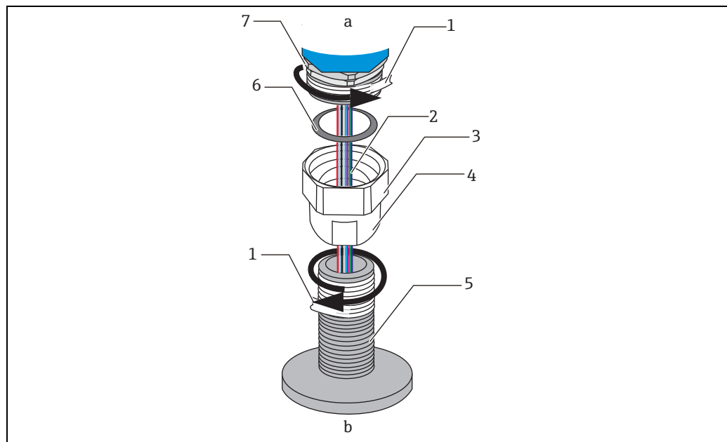
Figure 36: Connecting Threaded Type Connector
