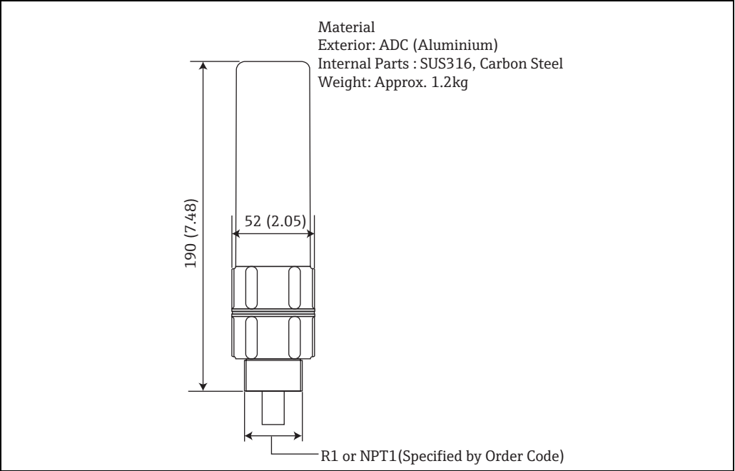
Figure 50: Top anchor dimensions, Unit of measurement: mm (in)
