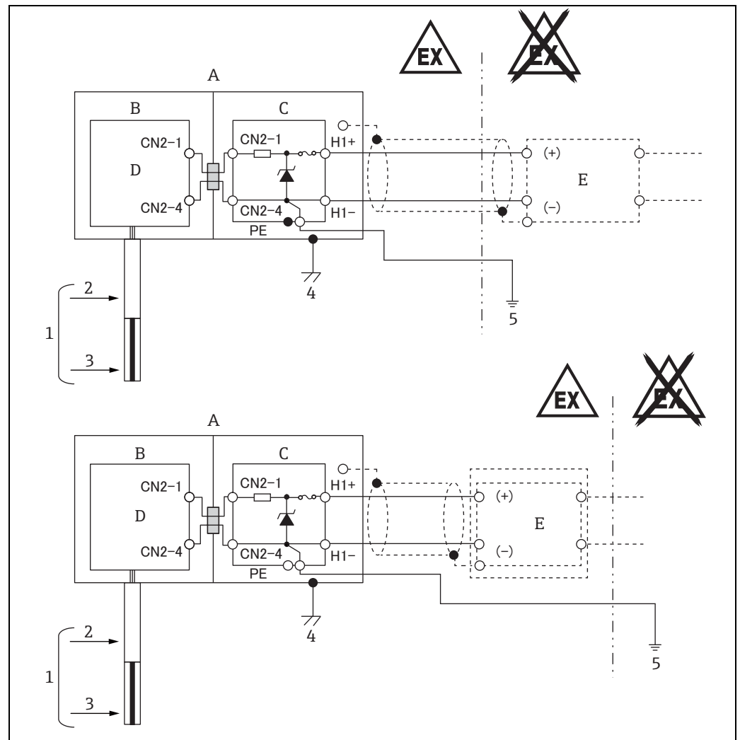
Figure 39: Connecting diagram
