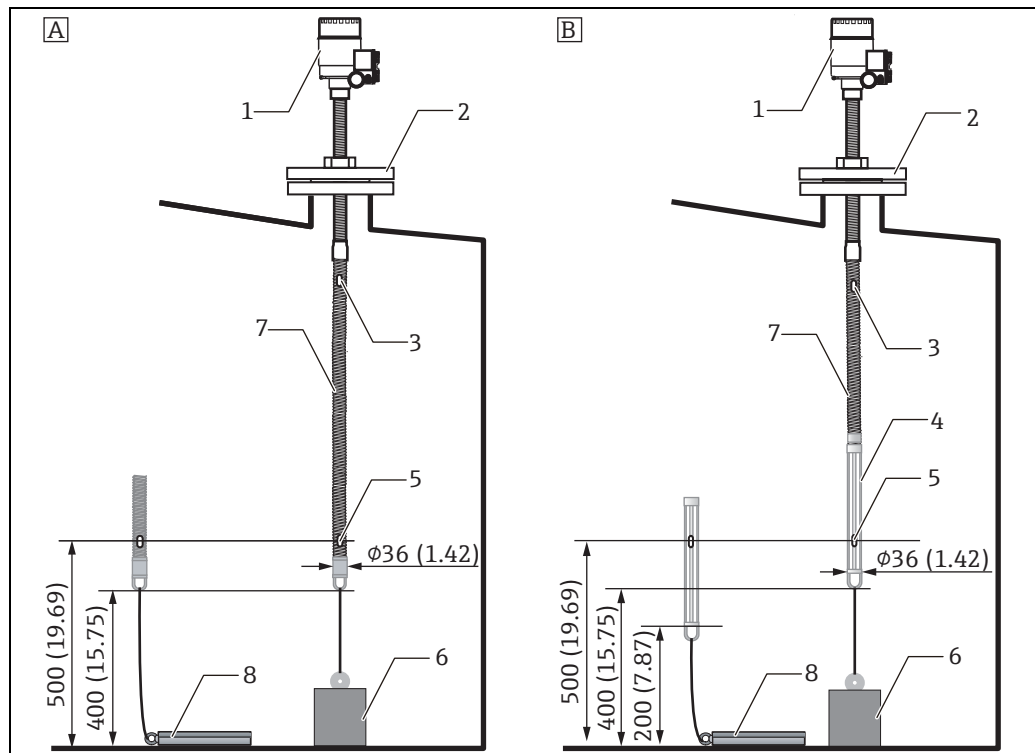
Figure 27: Anchor weight method, Unit of measurement: mm (in)
