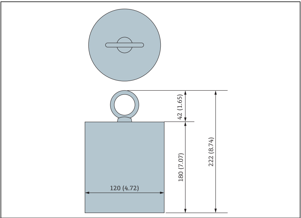
Figure 47: Anchor Weight for High Profile, Option B, Unit of measurement: mm (in)
