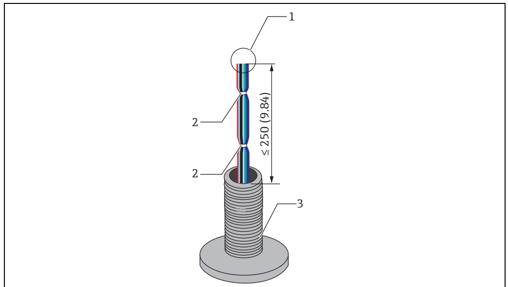
Figure 35: Tying cable
