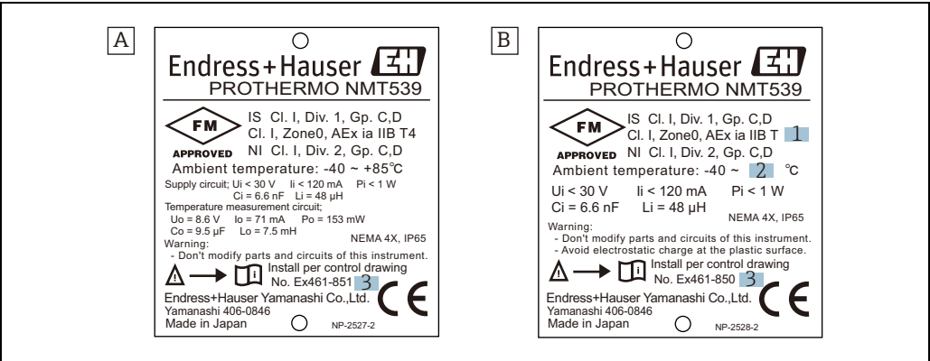
Figure 6: FM approval nameplate
