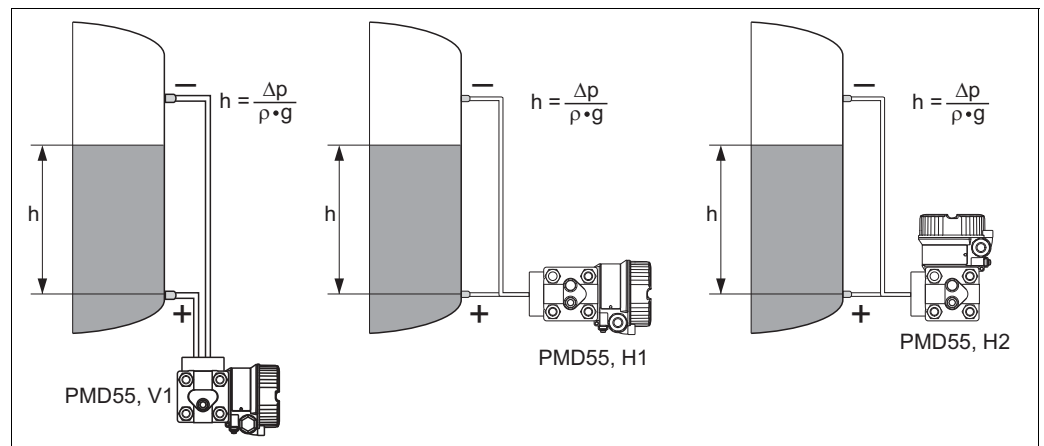
Level measurement with Deltabar M; left: V1 version; vertical impulse lines; 90° alignment middle: H1 version; horizontal impulse lines; 180° alignment right: H2 version; horizontal impulse lines; 90° alignment
