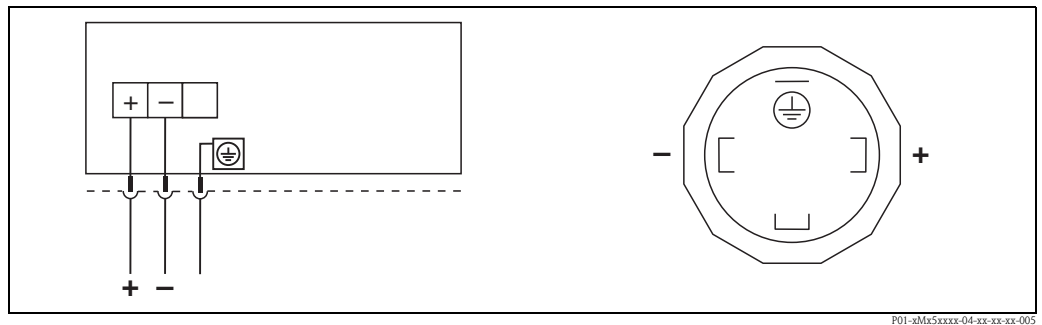
Left: electrical connection for devices with a valve connector Right: view of the connector at the device
