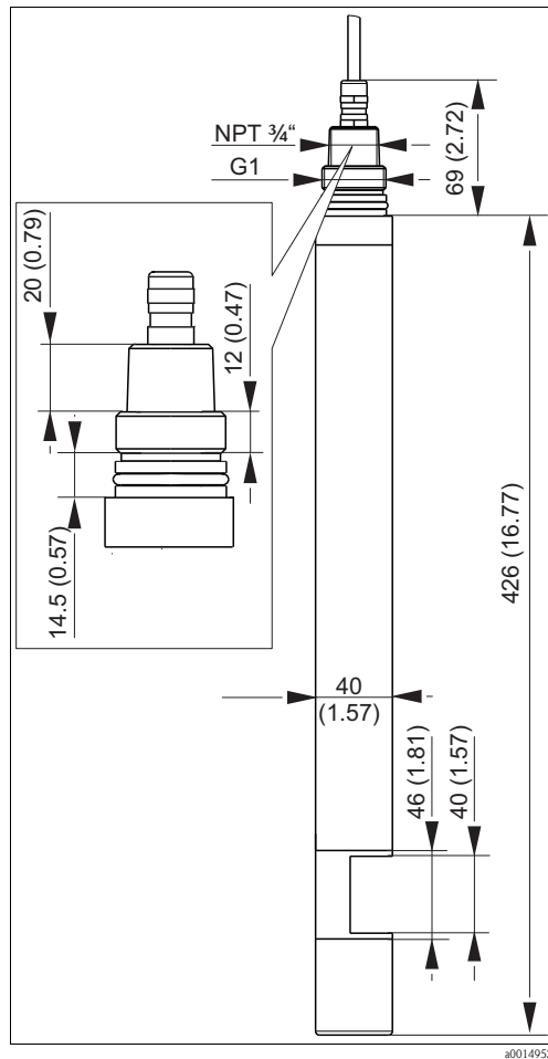
Fig. 3: Dimensions of CAS51D (40 mm gap)
