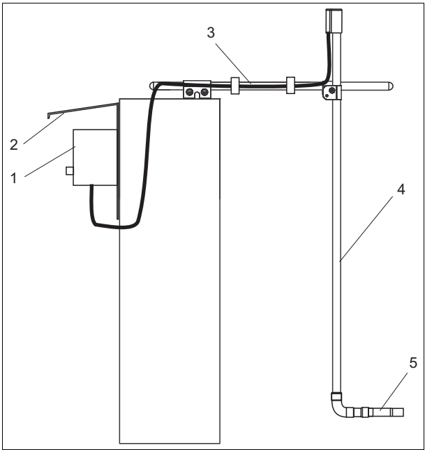
Fig. 5: Measuring system with immersion assembly (example)
