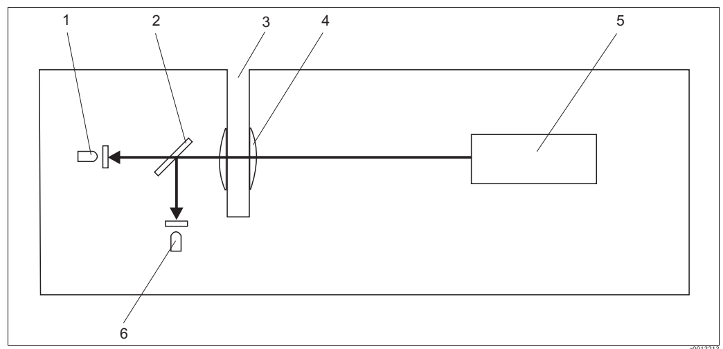
Fig. 20: Principal mode of operation of the nitrate sensor
