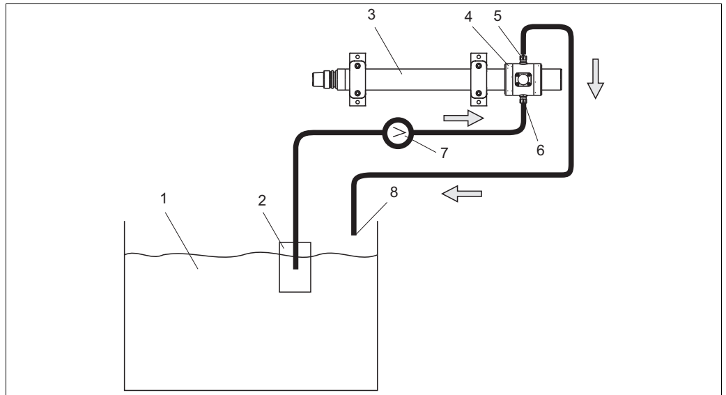
Fig. 15: Flow assembly with open outlet
