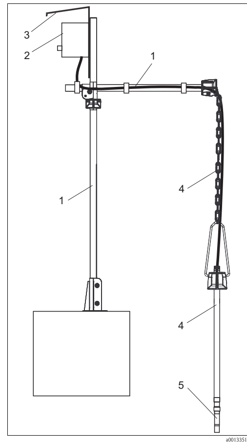
Fig. 10: Chain retainer on upright post
