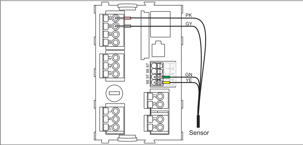
Fig. 19: Sensor connection
