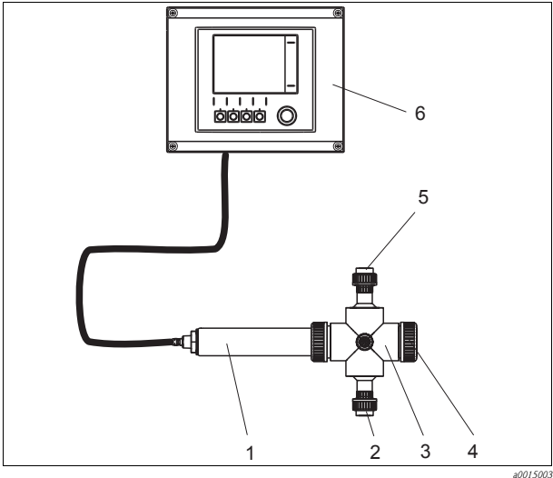
Fig. 6: Measuring system with flow assembly (example)
