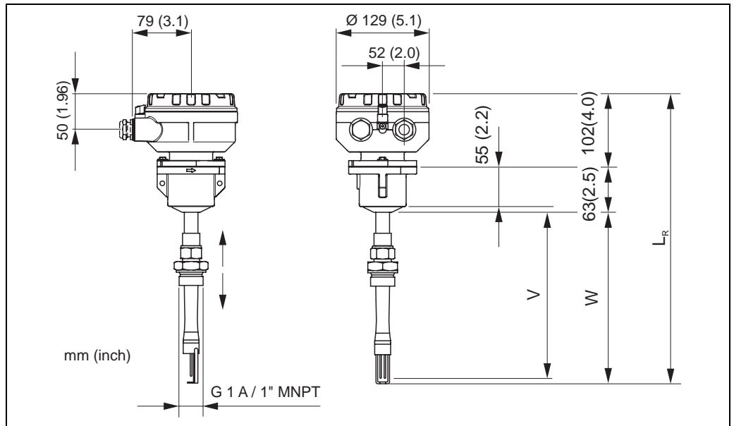
t-mass 65I: Remote sensor housing insertion version
