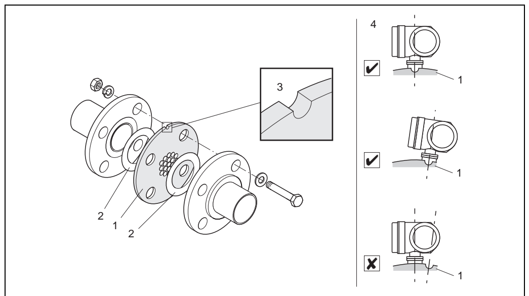
Flow conditioner mounting arrangement (example)
