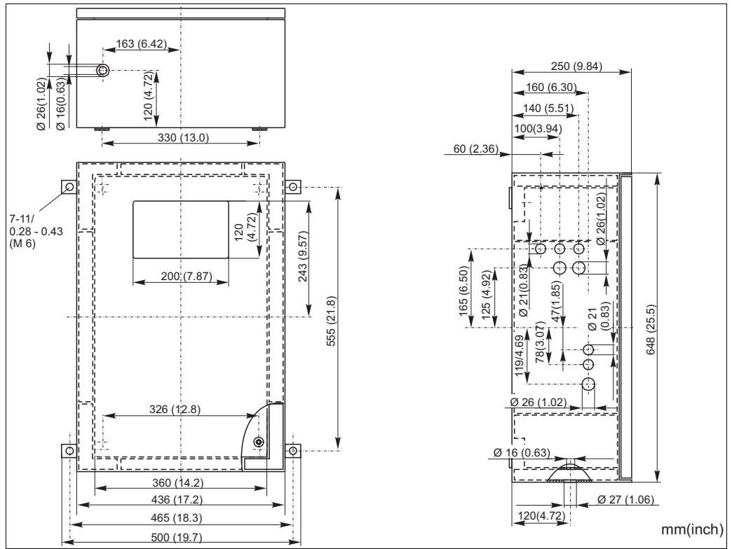
Fig. 3: GFR version
