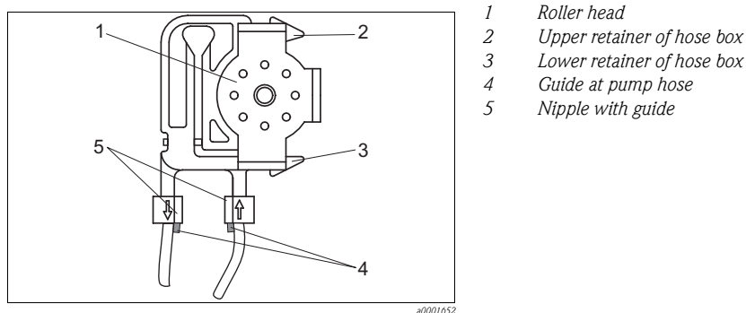
Fig. 22: Reagent pump
