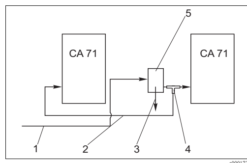
Fig. 14: Installation example
