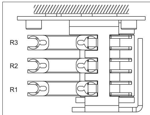
Fig. 13: Reagent pump, top view
