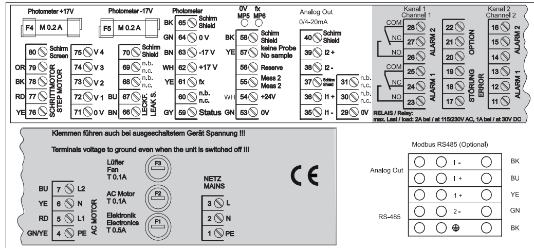
Fig. 17: Example of the connection sticker
