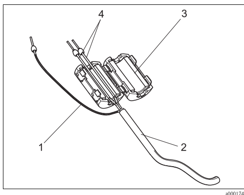
Fig. 19: Interference protection of the signal cable
