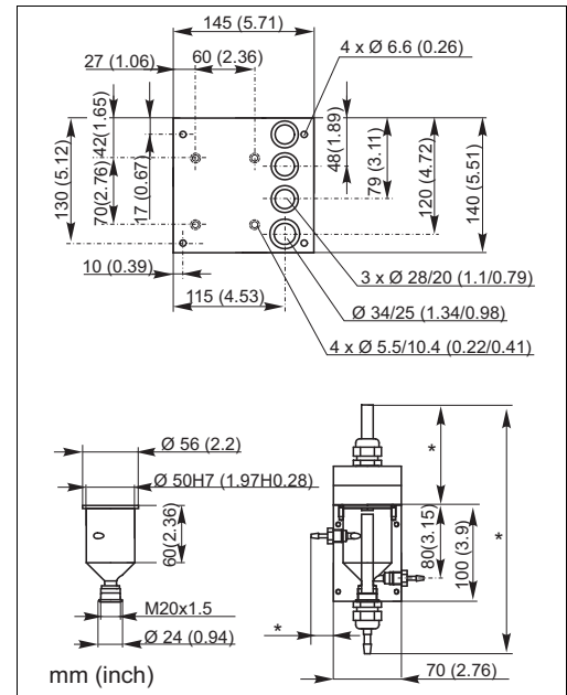
Fig. 7: Collecting vessel dimensions
