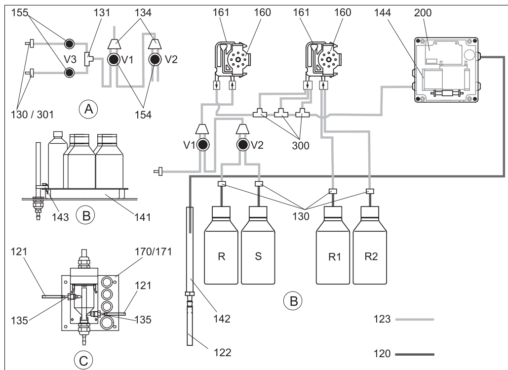
Fig. 26: Overview parts
