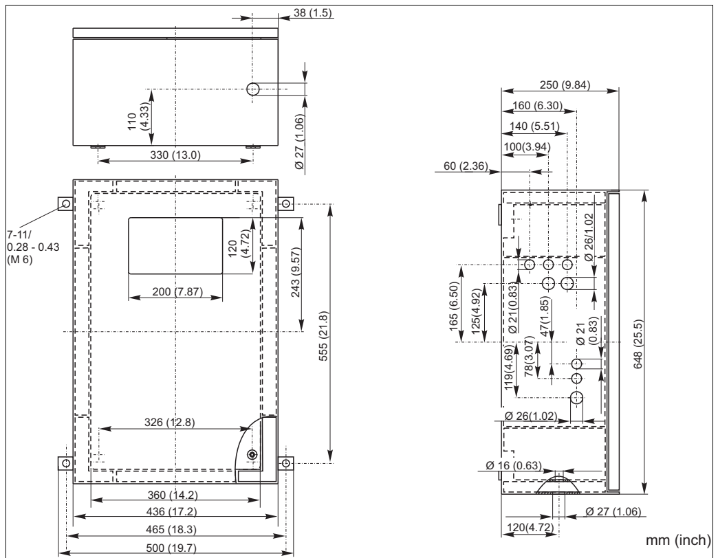
Fig. 4: GFR version
