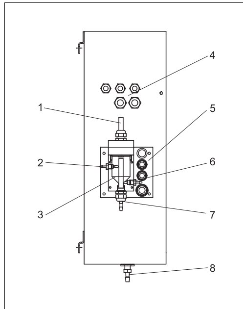
Fig. 6: Collecting vessel at analyzer (optional)
