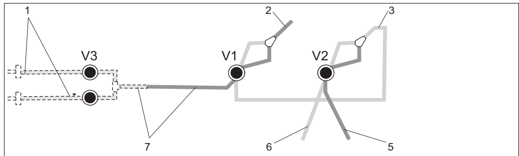
Fig. 11: Valves and valve hoses CA71AM-A/B/C
