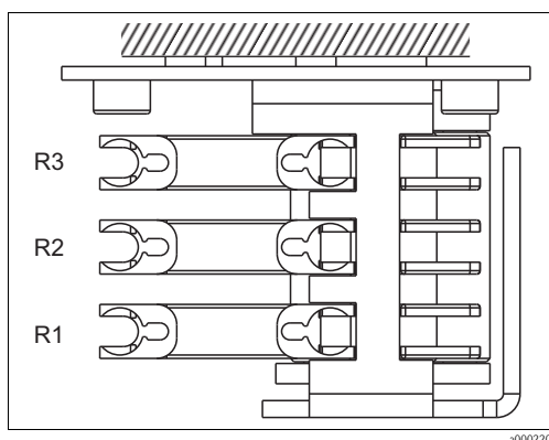
Fig. 23: Reagent pump, top view
