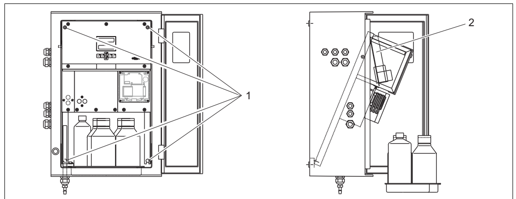
Fig. 16: Folding out the frame
