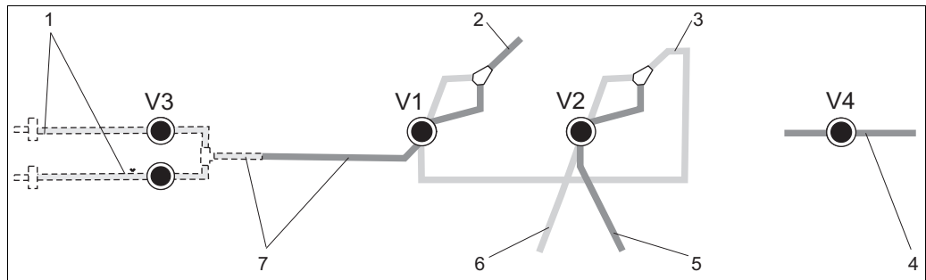
Fig. 12: Valves and valve hoses CA71AM-D
