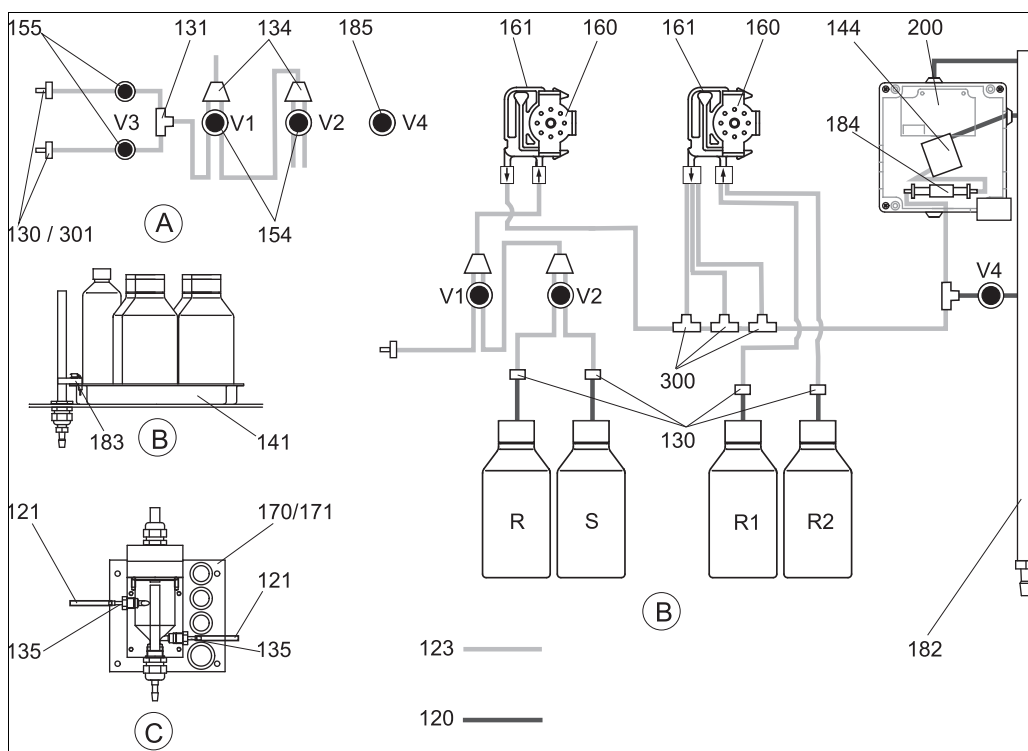
Fig. 27: Overview of spare parts
